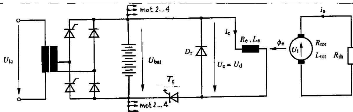
FREINAGE (1/4 locomotive 91).
